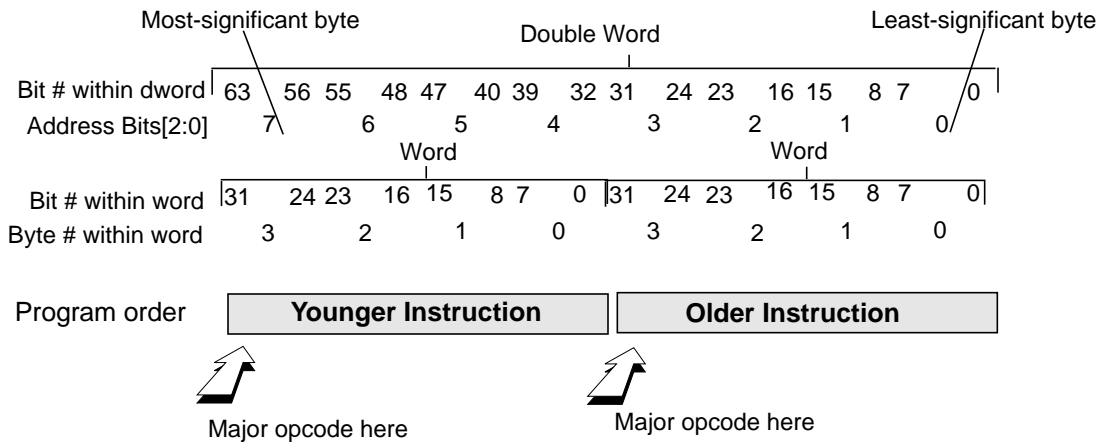
Figure 2-16 Two instructions placed in a 64-bit wide, little-endian memory
