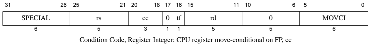
Figure 5-26 Condition Code, Register Integer FPU Instruction Format
