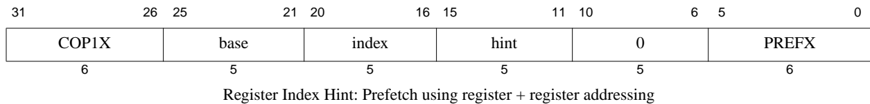
Figure 5-25 Register Index Hint FPU Instruction Format
