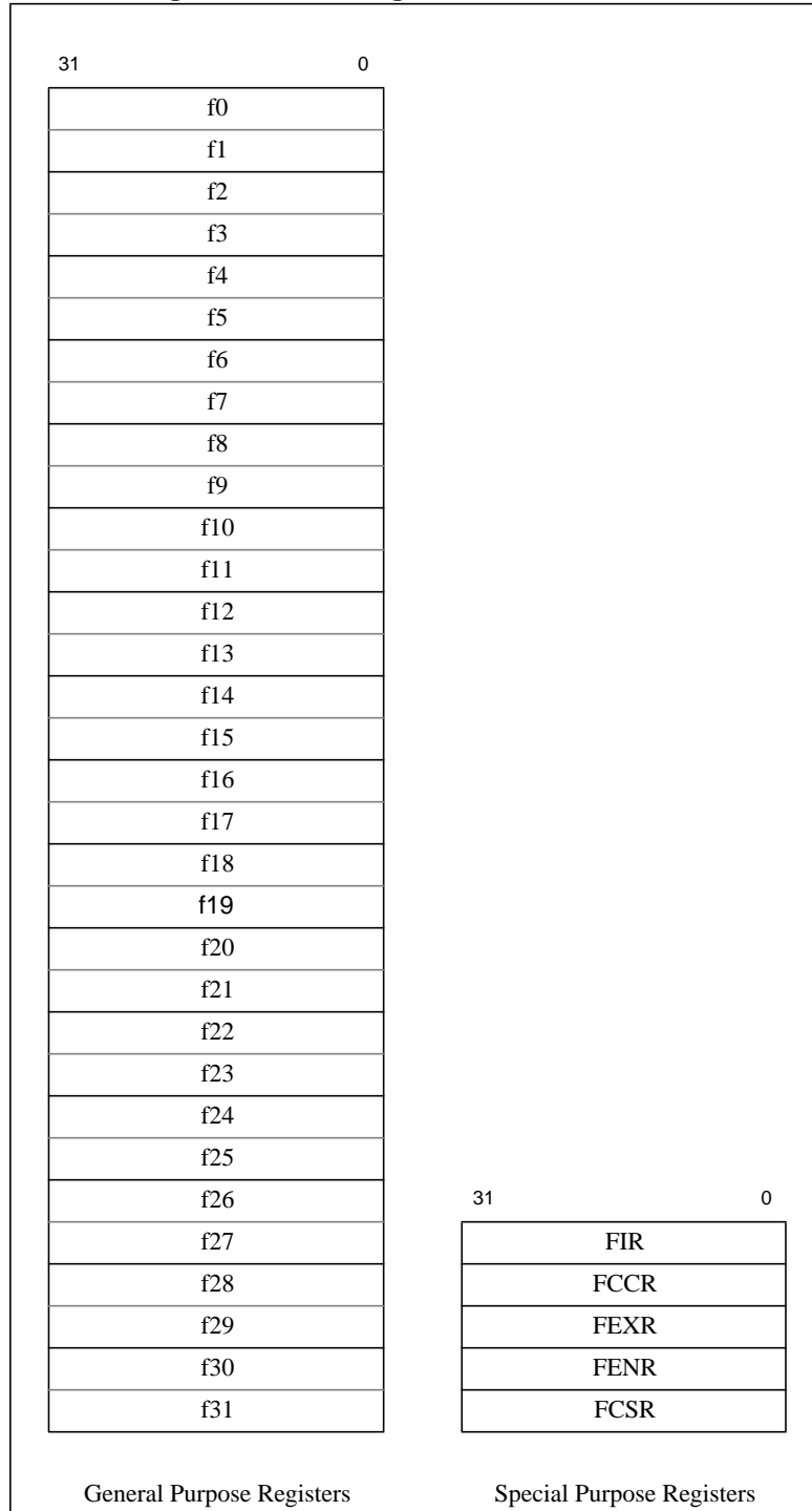
Figure 2-7 FPU Registers for a 32-bit FPU
