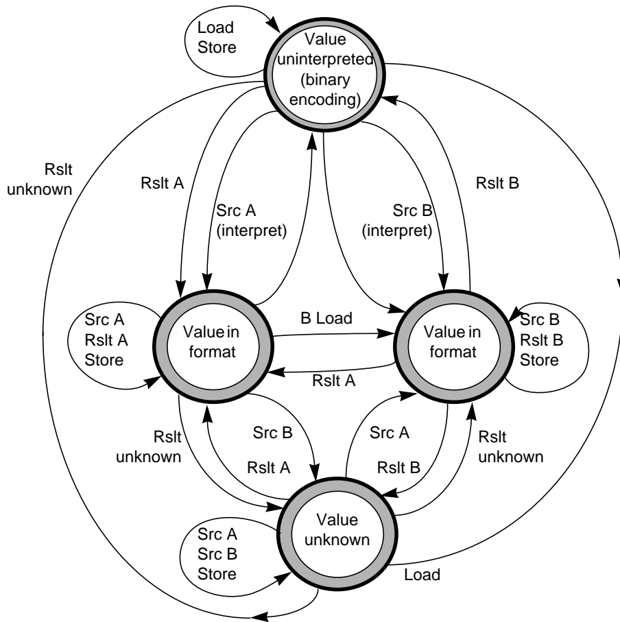
Figure 5-16 Effect of FPU Operations on the Format of Values Held in FPRs
