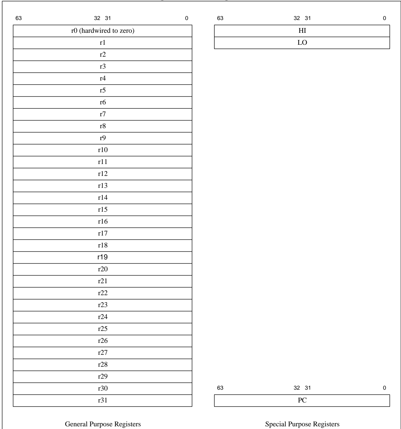
Figure 2-6 CPU Registers
